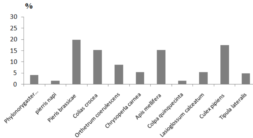
Figure 2: Centesimal Frequencies Species Trapped by the Butterfly Net
