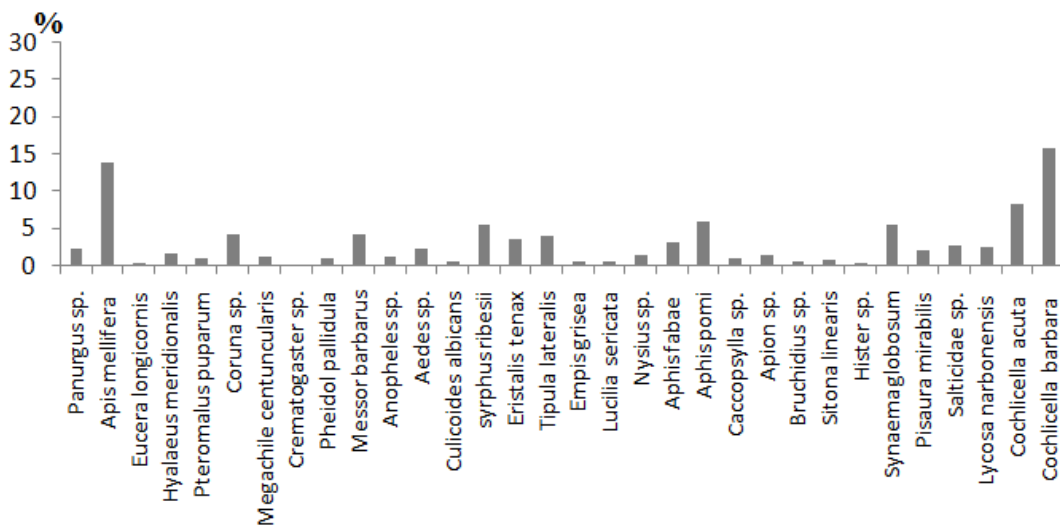
Figure 1: Centesimal Frequencies Species Trapped by the Sweep Net
