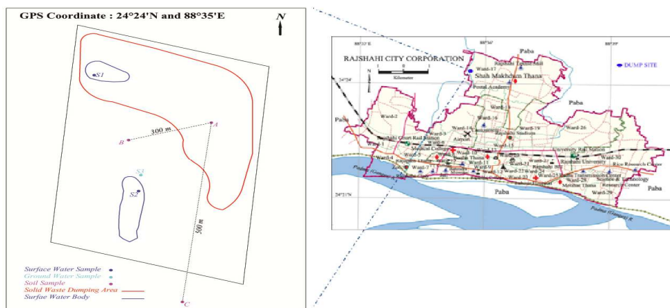
Figure 1: Soil and Water Sampling Location
